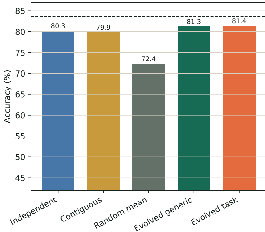
Qwen2.5-VL-3B-Instruct
