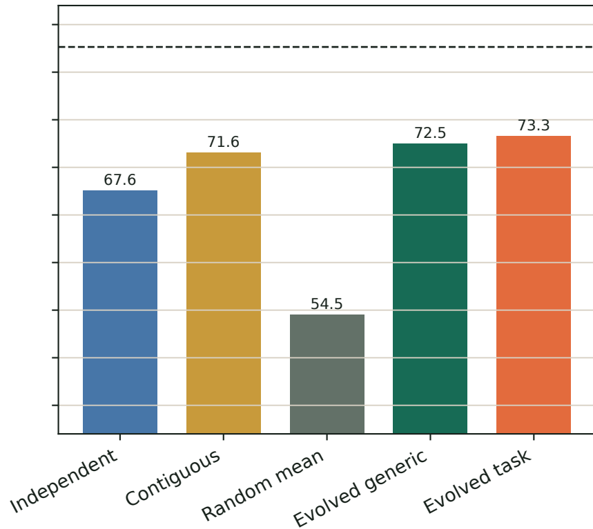
SmolVLM2-2.2B-Instruct
