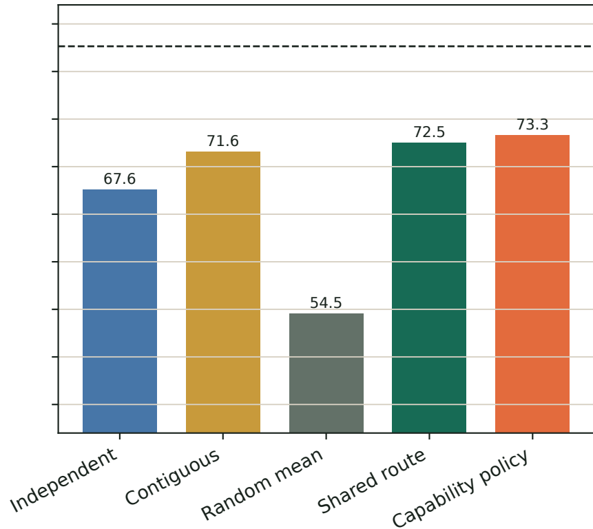
SmoIVLM2-2.2B-Instruct
