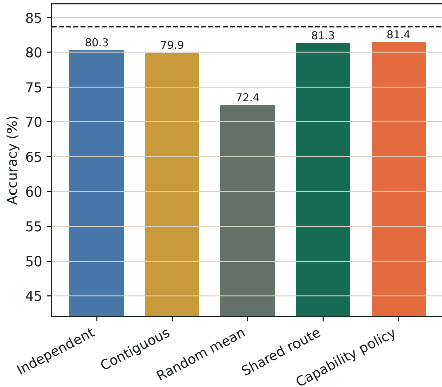
Qwen2.5-VL-3B-Instruct
