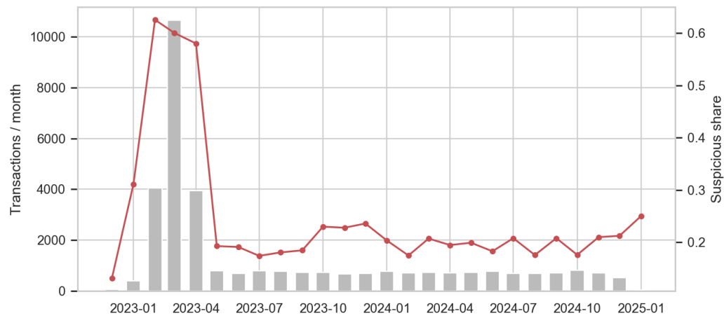
Transactions and suspicious rate by month.
