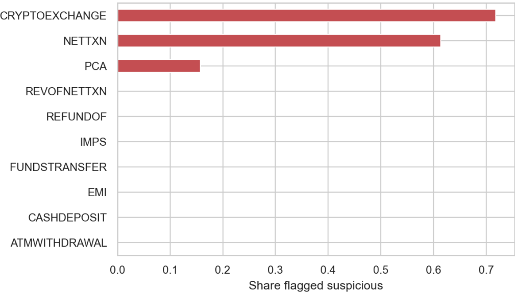
Suspicious rate by channel.
