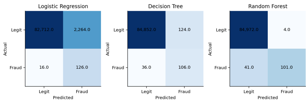
Confusion matrices of the three models.
