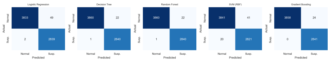
Confusion matrices of the tuned models.
