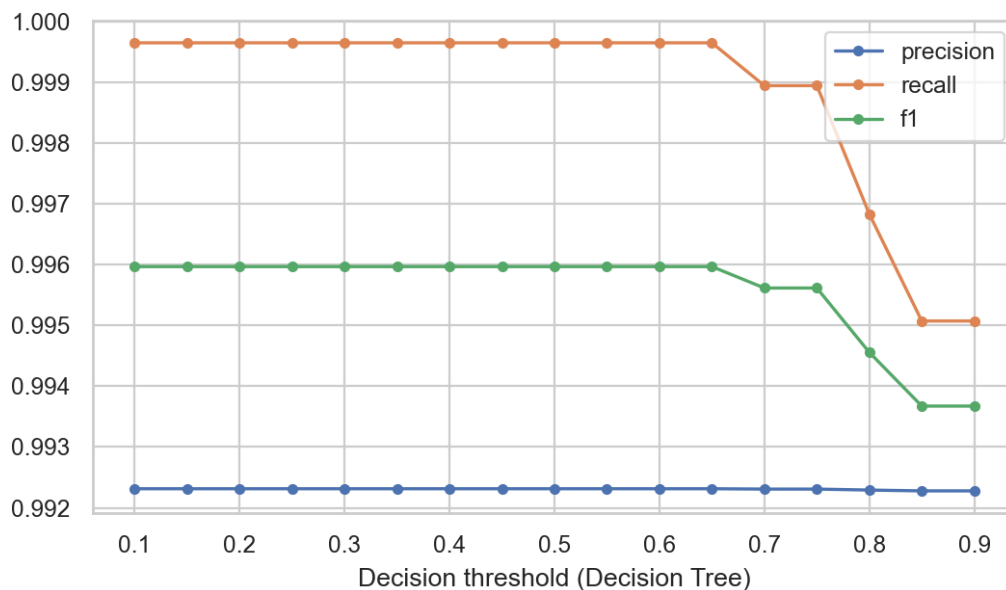
Precision and recall of the best model at different thresholds.
