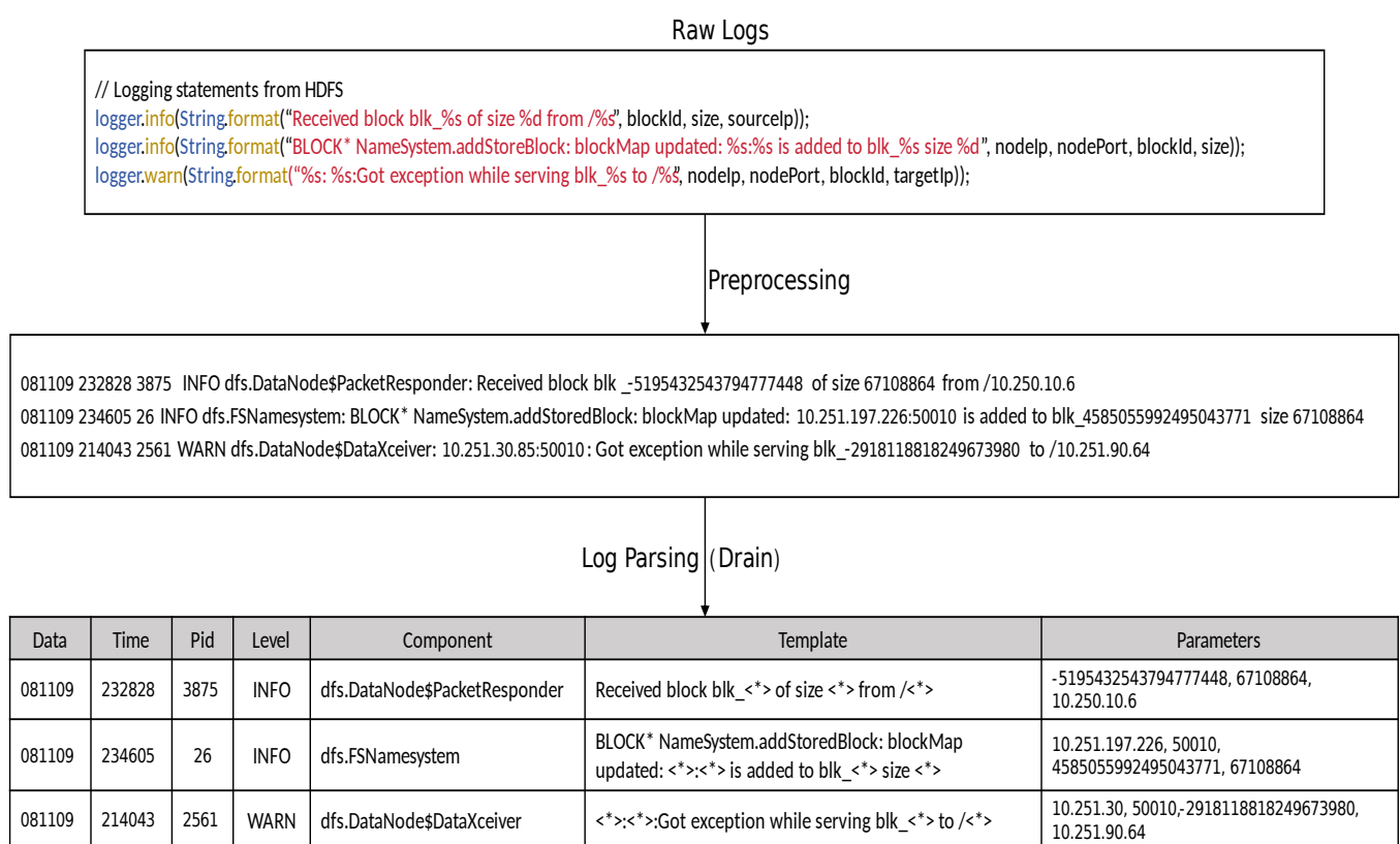
Figure 1. An example of an HDFS log and the corresponding log template event generated using the Drain log parsing method, where the variables in the log are replaced by placeholders <*> according to the template order.
