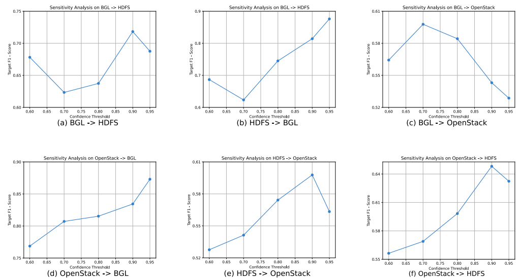
Figure 5. Sensitivity of the F1-score to the pseudo-label confidence threshold across all six domain adaptation scenarios. The results illustrate that no single threshold is optimal for all tasks, highlighting the necessity of adapting this hyperparameter to the specific characteristics of the target domain.
