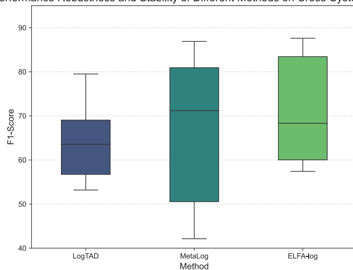
Figure 4. Performance Robustness and Stability of Different Methods on Cross-System Tasks. The box plot shows the distribution of F1-scores for each method across all six cross-system scenarios.
