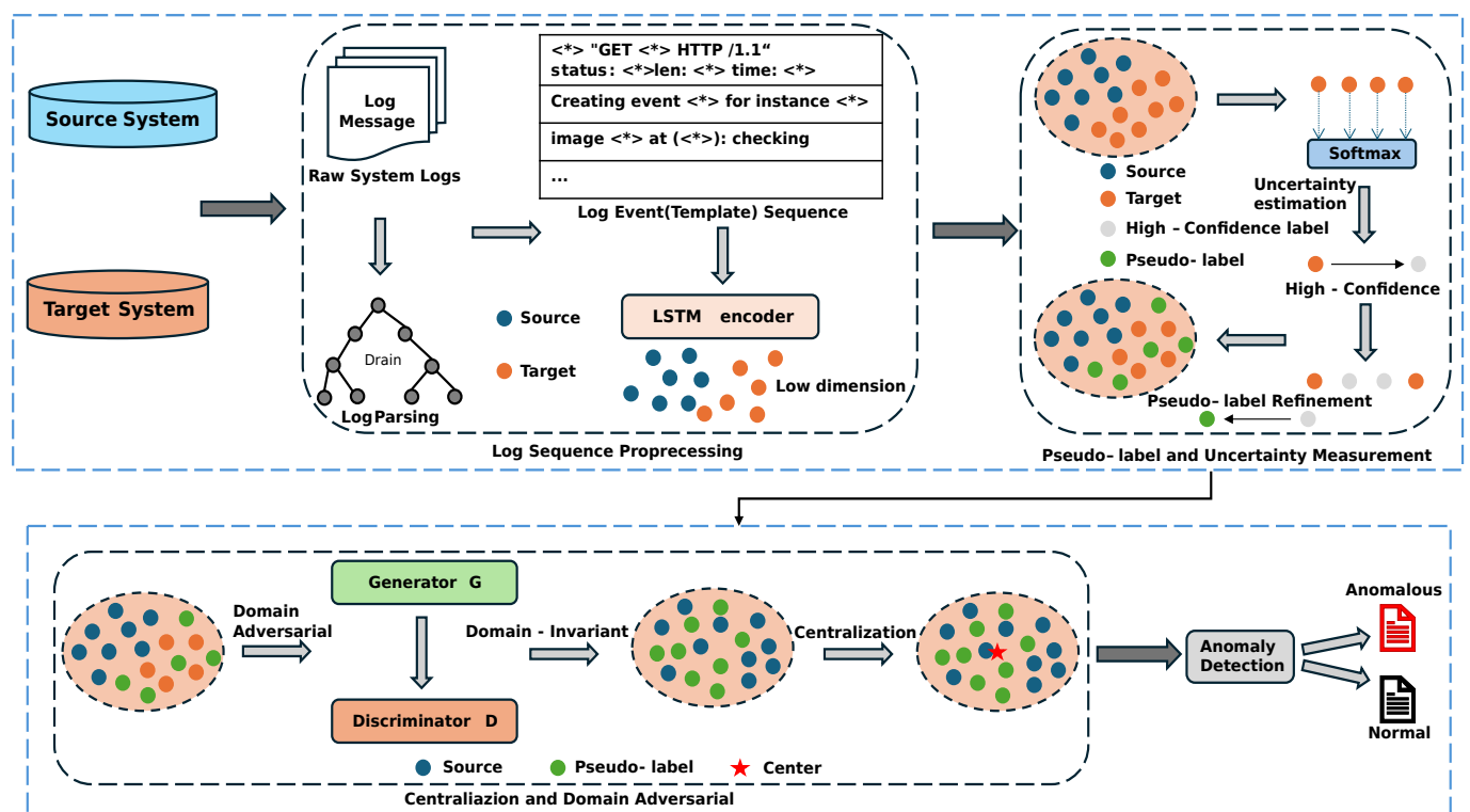
Figure 3. The Framework of ELFA-Log.
