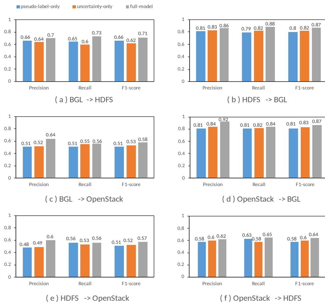
Figure 6. Ablation Studies Results.
