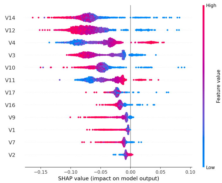
SHAP summary for Random Forest.
