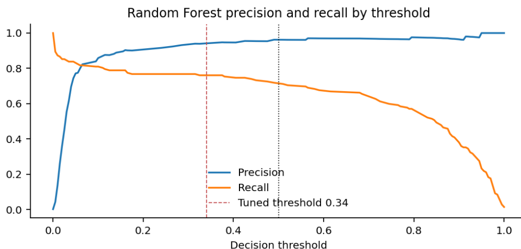
Random Forest precision and recall at different thresholds.
