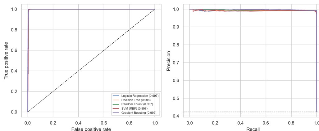
ROC and precision-recall curves on the test set.
