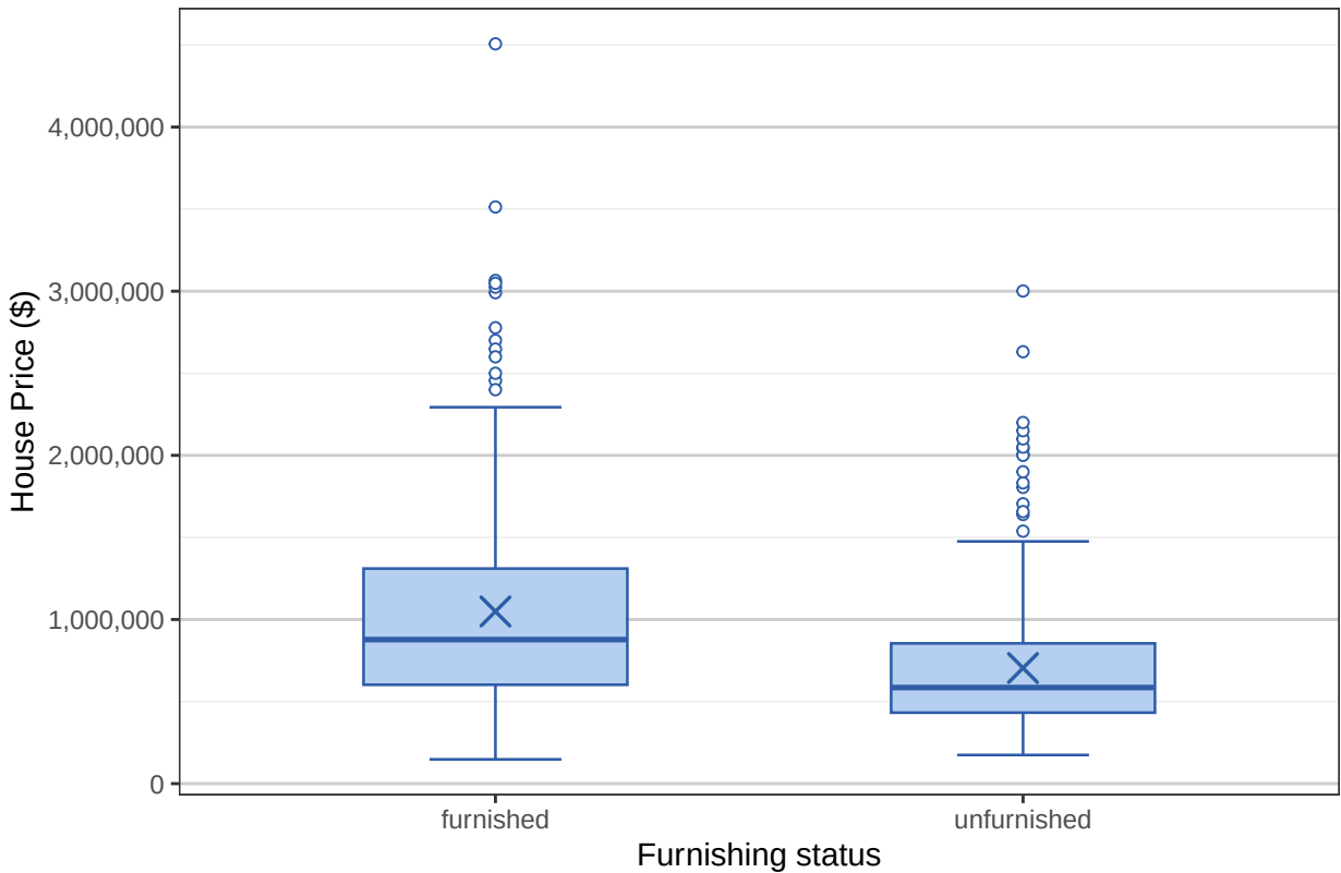
Distribution of house price according to furnishing status (n = 545)
