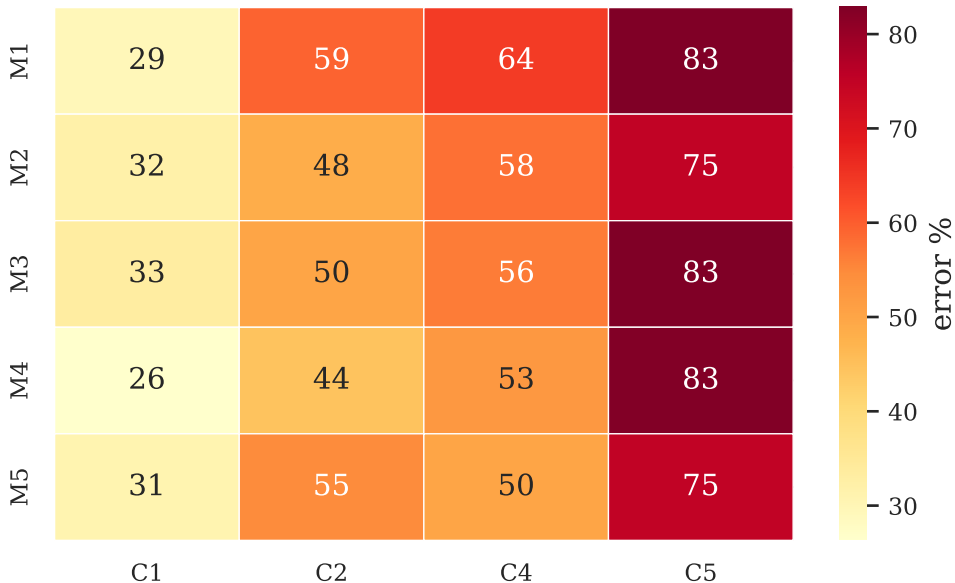
Error rate by model × condition
