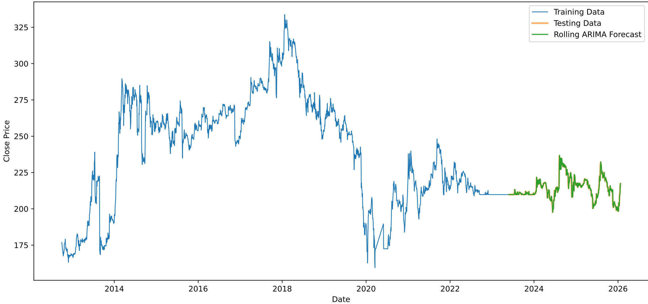
Rolling ARIMA(1,1,1) Forecast Illustration (SQURPHARMA)
