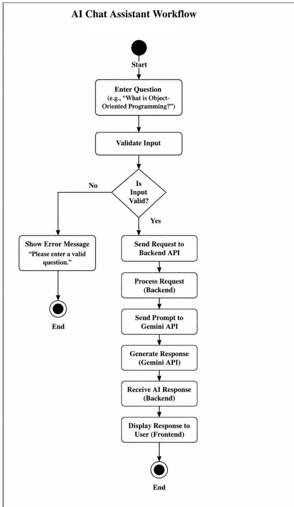
Fig. : Activity Diagram (AI Chat Assistant Workflow)
