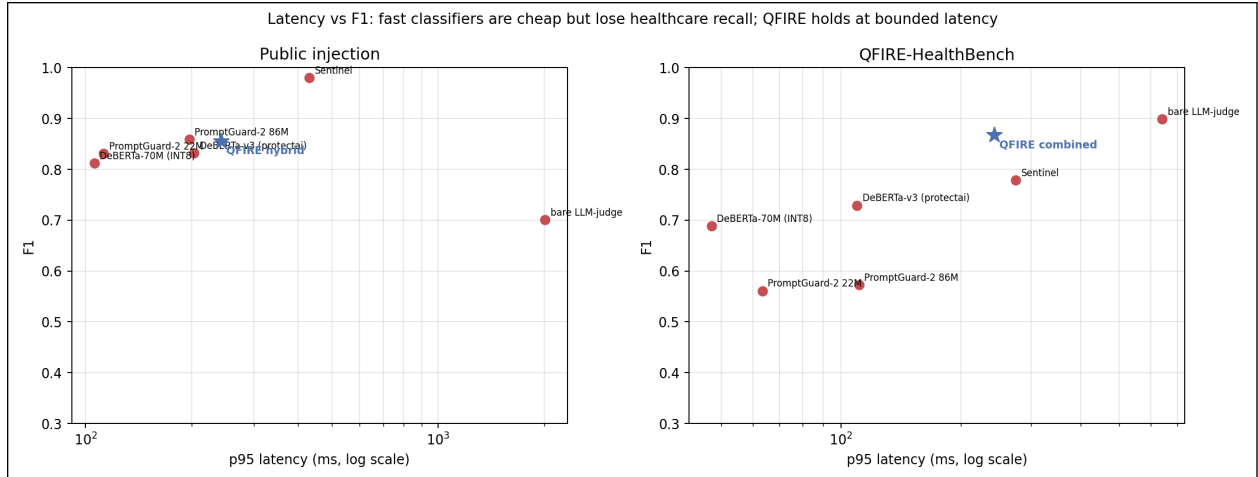
Figure 6: Latency (p95, log scale) vs F1 for every detector, on public injection (left) and QFIRE-HealthBench (right). Compressed classifiers (DeBERTa-70M, PromptGuard-2 22M) are cheap and competitive on injection but, like all generic classifiers, lose recall on healthcare; the bare LLM-judge is slowest. QFIRE (★) holds high F1 at bounded latency on both—healthcare especially. QFIRE’s HealthBench point uses the hybrid-chain p95 as a latency proxy (the combined chain short-circuits, so it has no single classifier p95).
