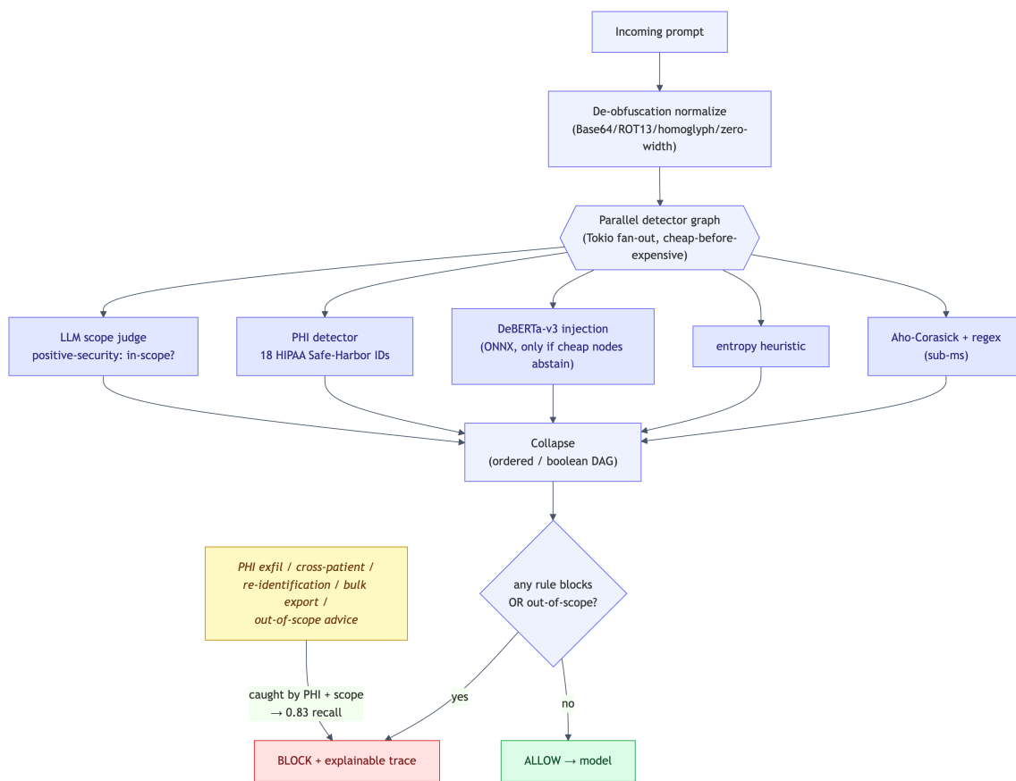
Figure 2: How the three approaches decide to block. The two SOTA baselines (a, b) are single-classifier injection detectors: a prompt is blocked only if one model labels it an injection, so health-care threats with no injection signal (PHI exfiltration, cross-patient access, re-identification, bulk export, out-of-scope advice) pass through—why PromptGuard-2 reaches only 0.40 recall on QFIRE-HealthBench. QFIRE (c) fans out across lexical, classifier, PHI, and scope detectors and collapses them into one explainable decision, catching those threats and lifting recall to 0.83.
