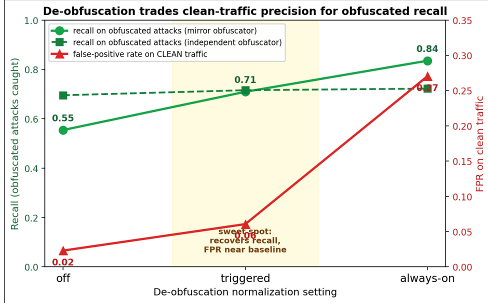
Figure 8: De-obfuscation trade-off across settings (off → triggered → always-on) for a mirror and an independent obfuscator. Recall on obfuscated attacks (green) rises with normalization while clean-traffic FPR (red) stays near baseline until always-on spikes it to 0.27. Triggered is the sweet spot. (§5.3.1)
