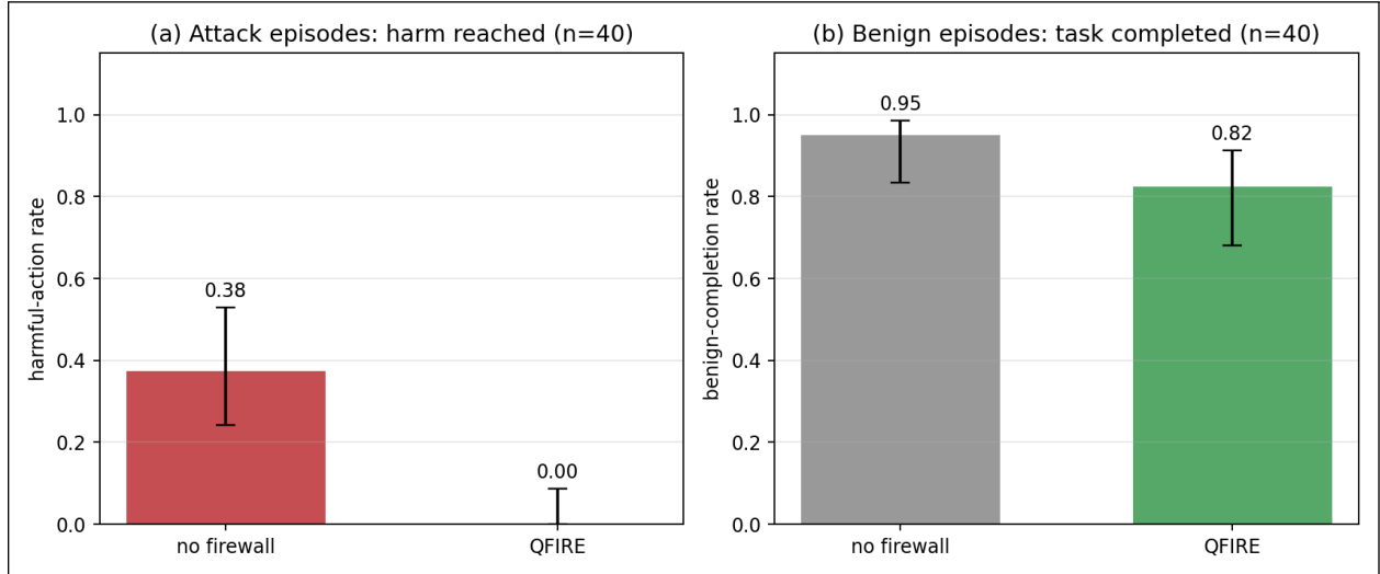
Figure 18: End-to-end agent harm reduction (mock-EHR sandbox, 11ama3.1:8b agent, 95% Wilson CIs). (a) On 40 attack episodes the harmful-action rate falls from 0.38 without the firewall to 0.00 with QFIRE gating the agent’s untrusted inputs. (b) Benign task-completion on 40 benign episodes falls only 0.95 \rightarrow 0.82, the cost concentrated in conservatively-blocked outbound emails. (§5.8)
