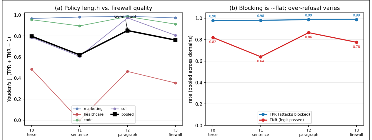
Figure 14: Policy-verbosity ablation (16 conditions, Llama 3.2 judge). (a) Youden's J vs. rung per domain (thin) and pooled (bold): non-monotone—the one-sentence rung dips, the structured paragraph peaks, the full firewall regresses. (b) Pooled true-positive rate (attacks blocked) is flat at 0.98 across all rungs, while the true-negative rate carries all the variation. Policy verbosity barely affects injection-blocking; its effect is on over-refusal. (§5.3.6)
