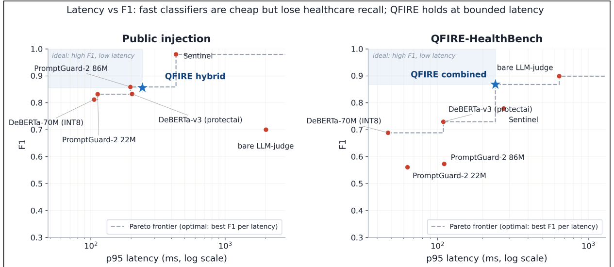
Figure 6: Latency (p95, log scale) vs F1 for every detector, on public injection (left) and QFIRE-HealthBench (right). Compressed classifiers (DeBERTa-70M, PromptGuard-2 22M) are cheap and competitive on injection but, like all generic classifiers, lose recall on healthcare; the bare LLM-judge is slowest. QFIRE (★) holds high F1 at bounded latency on both—healthcare especially. QFIRE’s HealthBench point uses the hybrid-chain p95 as a latency proxy (the combined chain short-circuits, so it has no single classifier p95).
