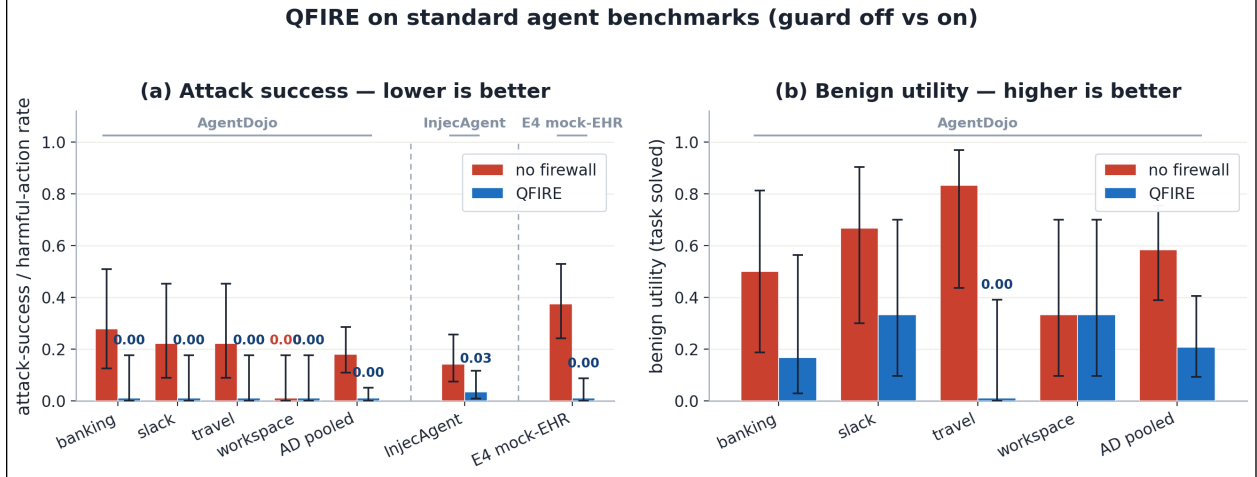
Figure 12: QFIRE on standard agent benchmarks, guard off (no firewall) vs. on (qwen3-coder:30b agent, important_instructions attack, 95% Wilson CIs). (a) Attack success: Targeted ASR per AgentDojo suite and pooled, InjecAgent attack-success, and the E4 mock-EHR harmful-action rate for reference; QFIRE drives AgentDojo ASR to 0 and cuts InjecAgent ASR \sim 4\times . (b) Benign utility (AgentDojo): the over-refusal cost of a broad per-suite domain scope.
