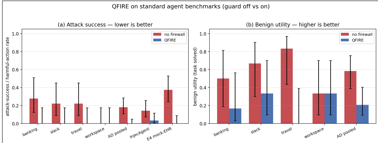
Figure 11: QFIRE on standard agent benchmarks, guard off (no firewall) vs. on ( qwen3-coder:30b agent, important_instructions attack, 95% Wilson CIs). (a) Attack success: Targeted ASR per AgentDojo suite and pooled, InjecAgent attack-success, and the E4 mock-EHR harmful-action rate for reference; QFIRE drives AgentDojo ASR to 0 and cuts InjecAgent ASR \sim 4\times . (b) Benign utility (AgentDojo): the over-refusal cost of a broad per-suite domain scope.
