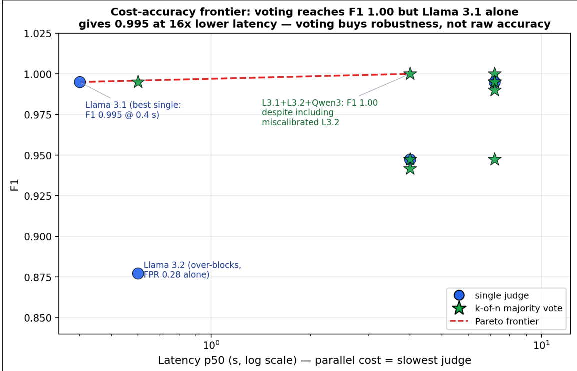
Figure 9: Cost-accuracy frontier: every single judge and every k -of- n majority vote in F1 \times \text{latency} space (latency = slowest member, log scale). The F1=1.000 ensembles include the miscalibrated Llama 3.2, whose false-positives are outvoted—voting buys robustness , not raw accuracy.
