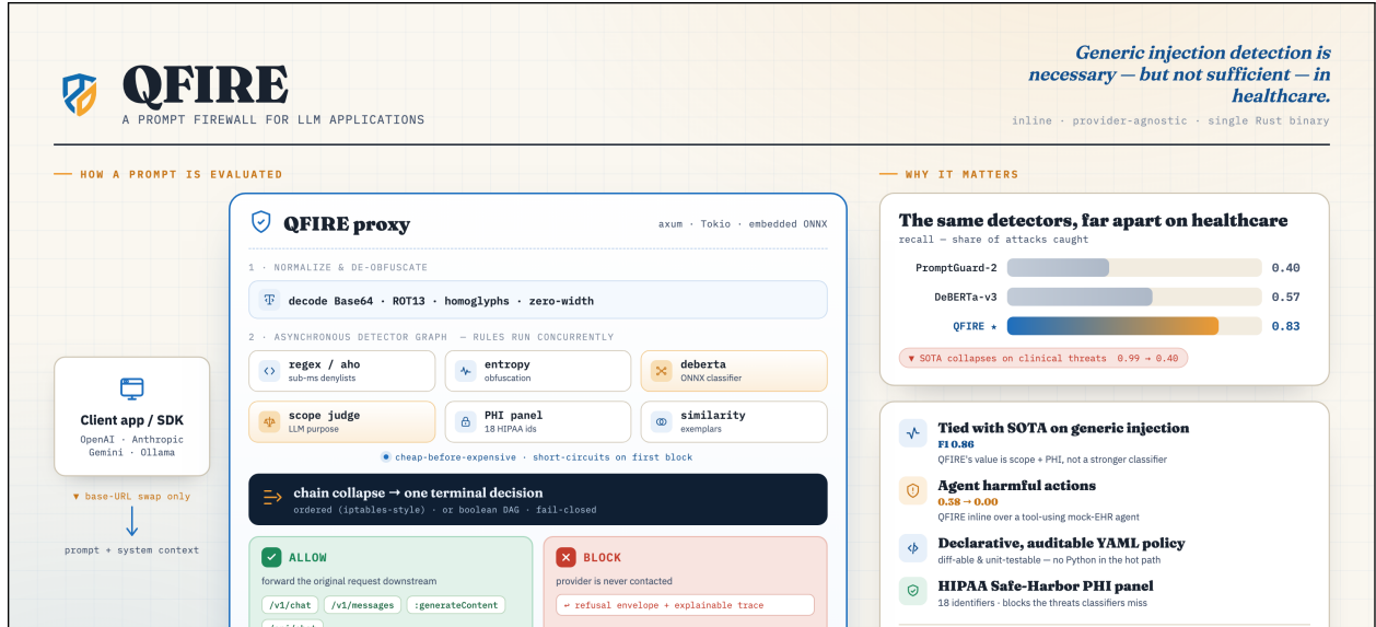
Figure 4: QFIRE at a glance. Left: the request path—a client SDK reaches QFIRE by swapping only its base URL; the proxy normalizes and de-obfuscates the prompt, runs an asynchronous detector graph (regex/Aho-Corasick, entropy, a local DeBERTa ONNX classifier, an LLM scope-judge, an 18-identifier HIPAA PHI panel, and exemplar similarity) cheap-before-expensive, and collapses the per-rule verdicts into one terminal decision. On ALLOW the original request is forwarded to the provider; on BLOCK it returns a refusal envelope and never contacts the provider, and every decision is appended to an immutable audit log. Right: the headline value—tied with SOTA on generic injection (F1 0.86) yet holding 0.83 recall on healthcare, where the same classifiers collapse to 0.40.
