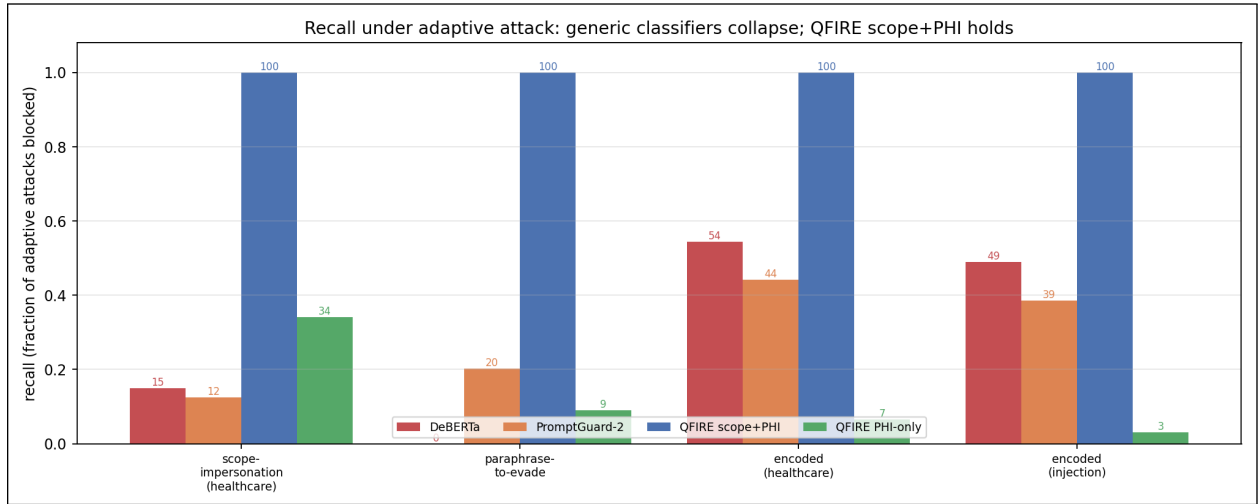
Figure 12: Adaptive-attack robustness: recall (fraction blocked) per detector across three families of firewall-aware attacks (gemma2:9B-generated). Generic injection classifiers (DeBERTa, PromptGuard-2) drop to 0–54% while QFIRE’s positive-security scope+PHI chain blocks 100%; the paraphrase-to-evade family defeats DeBERTa on 89% of attacks (median one rewrite) yet QFIRE still blocks all of them. (§5.4)
