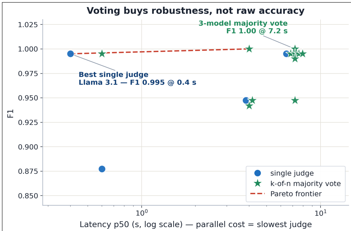
Figure 9: Cost-accuracy frontier: every single judge and every k -of- n majority vote in F1 \times latency space (latency = slowest member, log scale). The F1=1.00 ensembles include the miscalibrated Llama 3.2, whose false-positives are outvoted—voting buys robustness , not raw accuracy.
