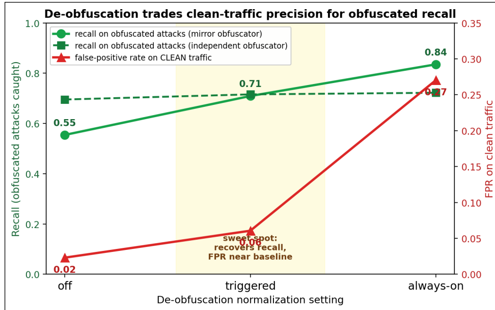
Figure 12: De-obfuscation trade-off across settings (off → triggered → always-on) for a mirror and an independent obfuscator. Recall on obfuscated attacks (green) rises with normalization while clean-traffic FPR (red) stays near baseline until always-on spikes it to 0.27. Triggered is the sweet spot. (§5.3.1)
