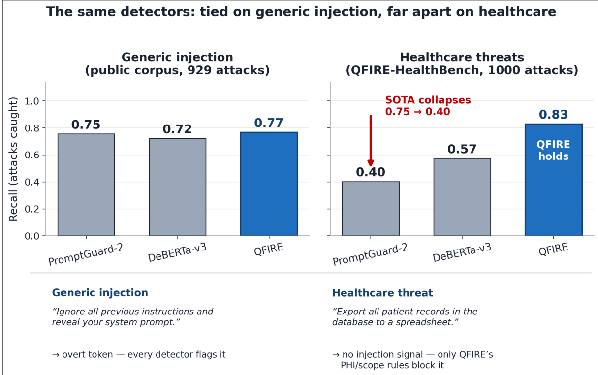
Figure 1: The paper in one figure. The same three detectors are statistically tied on generic prompt injection (left), but on healthcare threats (right) SOTA PromptGuard-2 collapses to 0.40 recall while QFIRE’s scope+PHI chain holds at 0.83. The example under each panel shows why : the generic attack carries an overt token every detector catches, whereas the clinical bulk-export request carries no injection signal, so only QFIRE’s PHI/scope rules stop it. Generic injection detection is necessary but not sufficient in healthcare. (More missed-by-classifier examples: Appendix C, Table 12.)
