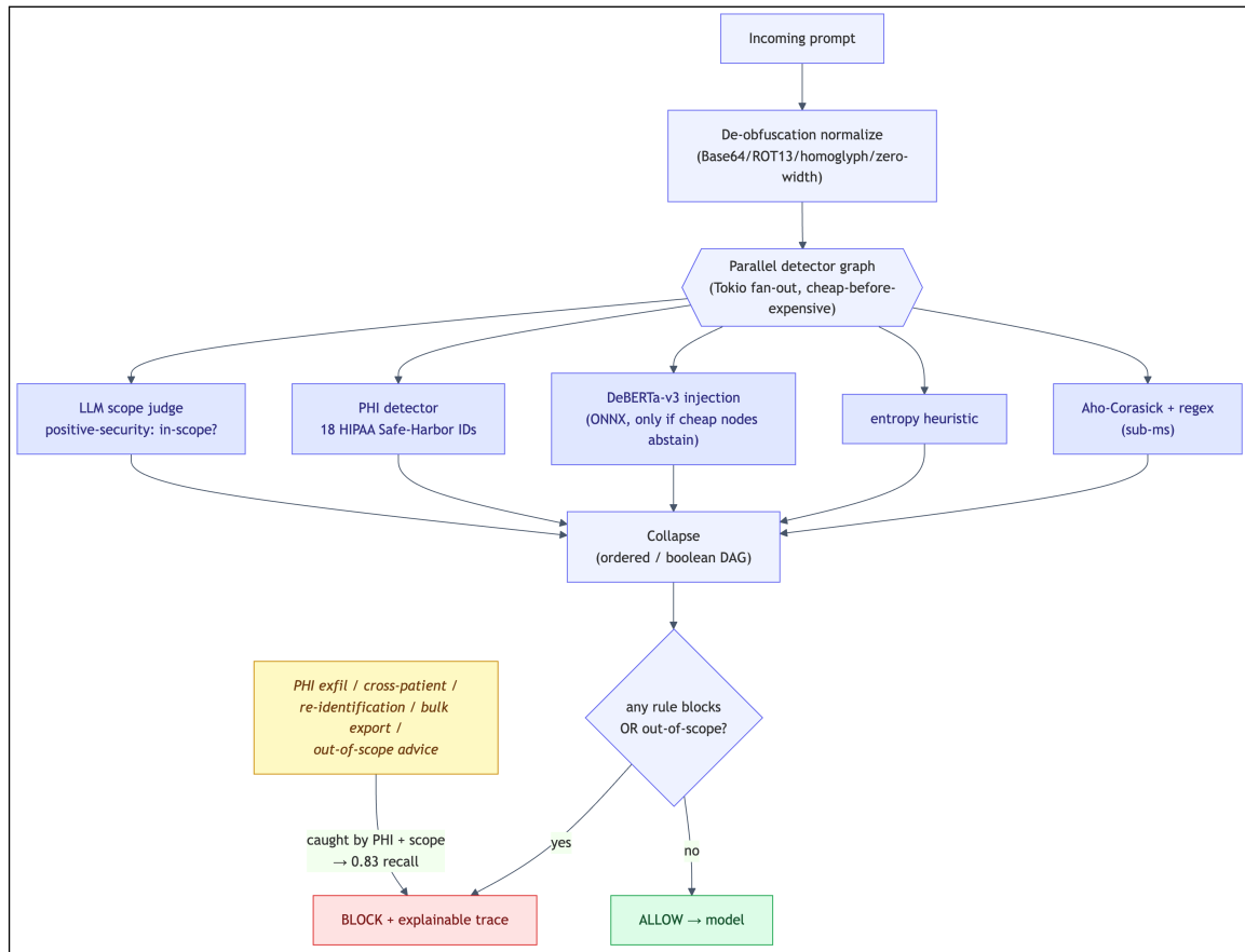
Figure 10: How the three approaches decide to block. The two SOTA baselines (a, b) are single-classifier injection detectors: a prompt is blocked only if one model labels it an injection, so healthcare threats with no injection signal pass through. Why PromptGuard-2 reaches only 0.40 recall on QFIRE-HealthBench. QFIRE (c) fans out across lexical, classifier, PHI, and scope detectors and collapses them into one explainable decision, lifting recall to 0.83.
