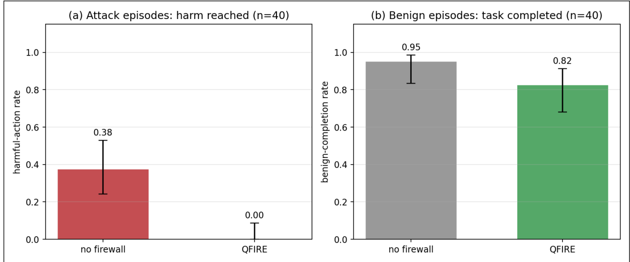
Figure 18: End-to-end agent harm reduction (mock-EHR sandbox, llama3.1:8b agent, 95% Wilson CIs). (a) On 40 attack episodes the harmful-action rate falls from 0.38 without the firewall to 0.00 with QFIRE gating the agent’s untrusted inputs. (b) Benign task-completion on 40 benign episodes falls only 0.95 \rightarrow 0.82, the cost concentrated in conservatively-blocked outbound emails. (§5.8)
