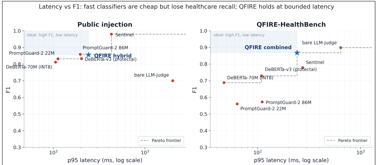
Figure 6: Latency (p95, log scale) vs F1 for every detector, on public injection (left) and QFIRE-HealthBench (right). Compressed classifiers (DeBERTa-70M, PromptGuard-2 22M) are cheap and competitive on injection but, like all generic classifiers, lose recall on healthcare; the bare LLM-judge is slowest. QFIRE (★) holds high F1 at bounded latency on both—healthcare especially. QFIRE’s HealthBench point uses the hybrid-chain p95 as a latency proxy (the combined chain short-circuits, so it has no single classifier p95).
