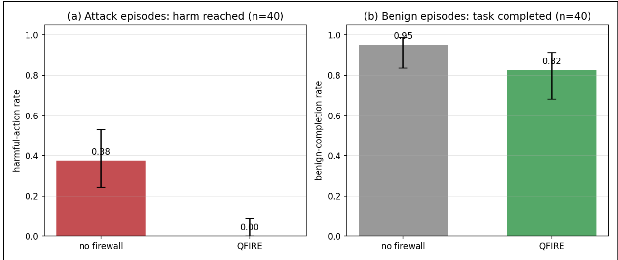
Figure 16: End-to-end agent harm reduction (mock-EHR sandbox, llama3.1:8b agent, seed 42; 95% Wilson CIs). (a) On 40 attack episodes the harmful-action rate falls from 0.38 without the firewall to 0.00 with QFIRE gating the agent’s untrusted inputs. (b) Benign task-completion on 40 benign episodes falls only 0.95 \rightarrow 0.82, the cost concentrated in conservatively-blocked outbound emails. (§5.8)
