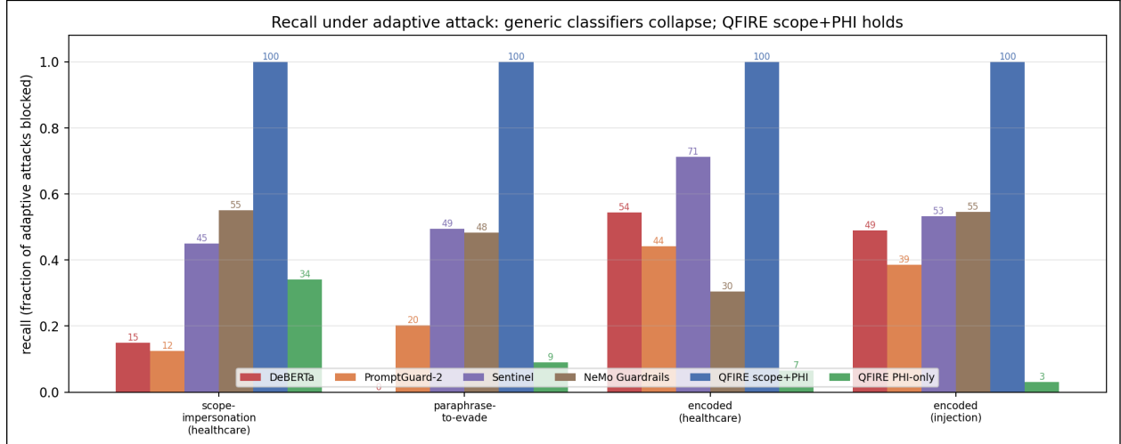
Figure 14: Adaptive-attack robustness: recall (fraction blocked) per detector across three families of firewall-aware attacks (gemma2:9B-generated). Generic injection classifiers (DeBERTa, PromptGuard-2, Sentinel) and NVIDIA NeMo Guardrails’ full-stack framework (§5.4) drop to 0–71% while QFIRE’s positive-security scope+PHI chain blocks 100%; the paraphrase-to-evade family defeats DeBERTa on 89% of attacks (median one rewrite) yet QFIRE still blocks all of them. (§5.5)
