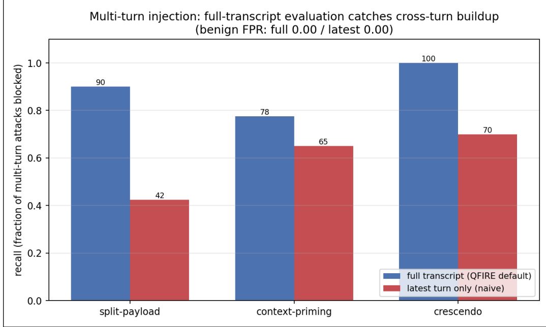
Figure 10: Multi-turn injection recall: QFIRE’s default full-transcript evaluation vs a naive latest-turn-only filter, per attack pattern (150 conversations, benign FPR 0.00 both modes). The full transcript reassembles split payloads and sees crescendo buildup the last turn alone misses.
