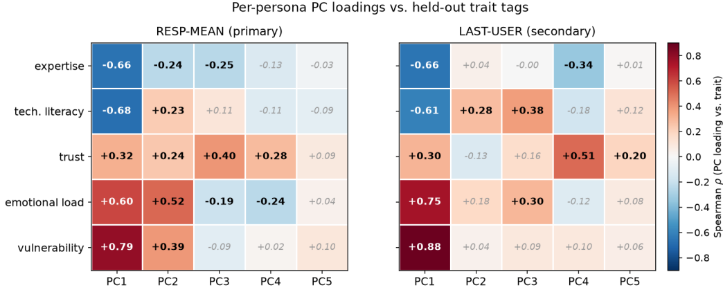
Figure 8: Which trait each principal component tracks. Spearman \rho between each persona’s loading on PC1–PC5 and each held-out 0–10 trait tag, for the RESP-MEAN (left) and LAST-USER (right) readouts. Significant cells (Benjamini–Hochberg q < 0.05 across the 25 cells of a panel) are bold; others are greyed. How to read it. (i) Down a column tells you which traits a PC correlates with, but note the five traits are one collinear bundle (Table 3)—a PC that tracks vulnerability necessarily also tracks emotional load, expertise and tech literacy, so a column is one bundle, not five independent loadings. (ii) Across a row is the cleaner reading, because the PCs are mutually orthogonal: it shows where a trait’s signal concentrates—almost entirely in PC1. (iii) PC1 is the only column that is dense, strong, and sign-stable across both readouts ; PC2–PC5 are weak, mostly non-significant, and disagree between readouts (e.g. PC2×emotional-load flips sign), consistent with their small variance shares (Table 10) and the readout-dependence discussed in §4. Each PC’s sign is arbitrary in PCA; every column is oriented so its largest-magnitude trait loads positive (PC1 toward vulnerability, matching the rest of the report), so only within-column signs are meaningful. Spearman \rho is near-identical to the Pearson r in the tables below (PC1×vuln \rho=0.79 vs. r=0.78 ).
