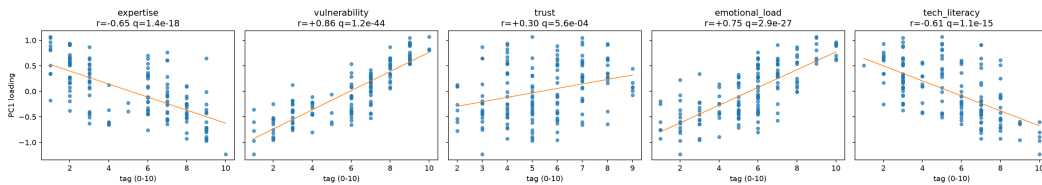
Figure 12: PC1 loading (LAST-USER) vs. each held-out tag. PC1~vulnerability reaches r=0.86 , q=1.2 \times 10^{-44} .
