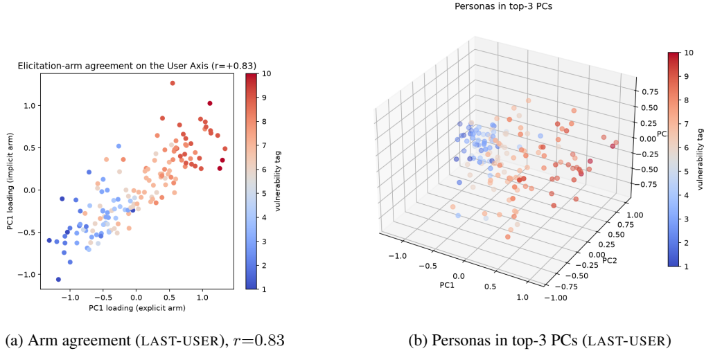
Figure 9: Elicitation-regime agreement and persona embedding for the secondary LAST-USER read-out.
