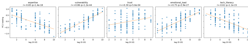
Figure 8: PC1 loading (LAST-USER) vs. each held-out tag. PC1~vulnerability reaches r=0.86 , q=1.2 \times 10^{-44} .
