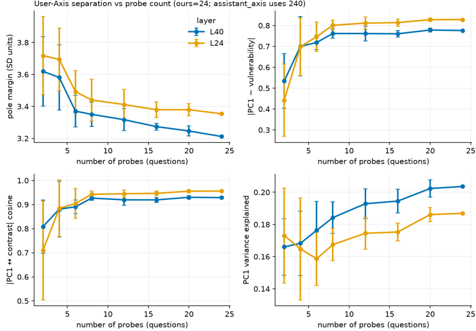
Figure 8: User-Axis separation vs. number of probes, both readouts (error bars = SD over R=8 random probe-subsets). The meaning metrics ( PC1 \sim \text{vulnerability} , PC1 \leftrightarrow \text{contrast cosine} ) plateau by \sim 8 probes; our 24 (and the parent’s 240) lie on the flat region.
