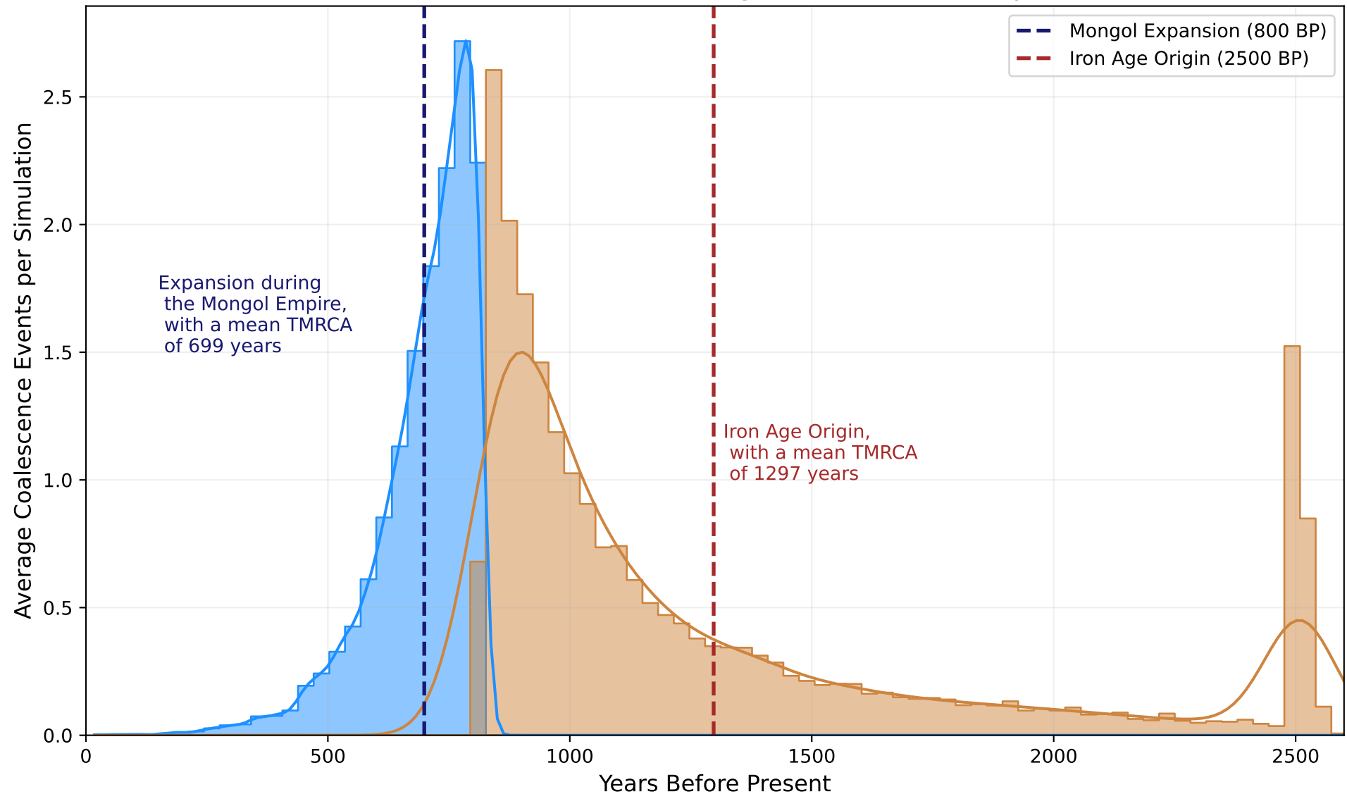
Coalescence Events in the Iron Age Scenario (1000 replicates)
