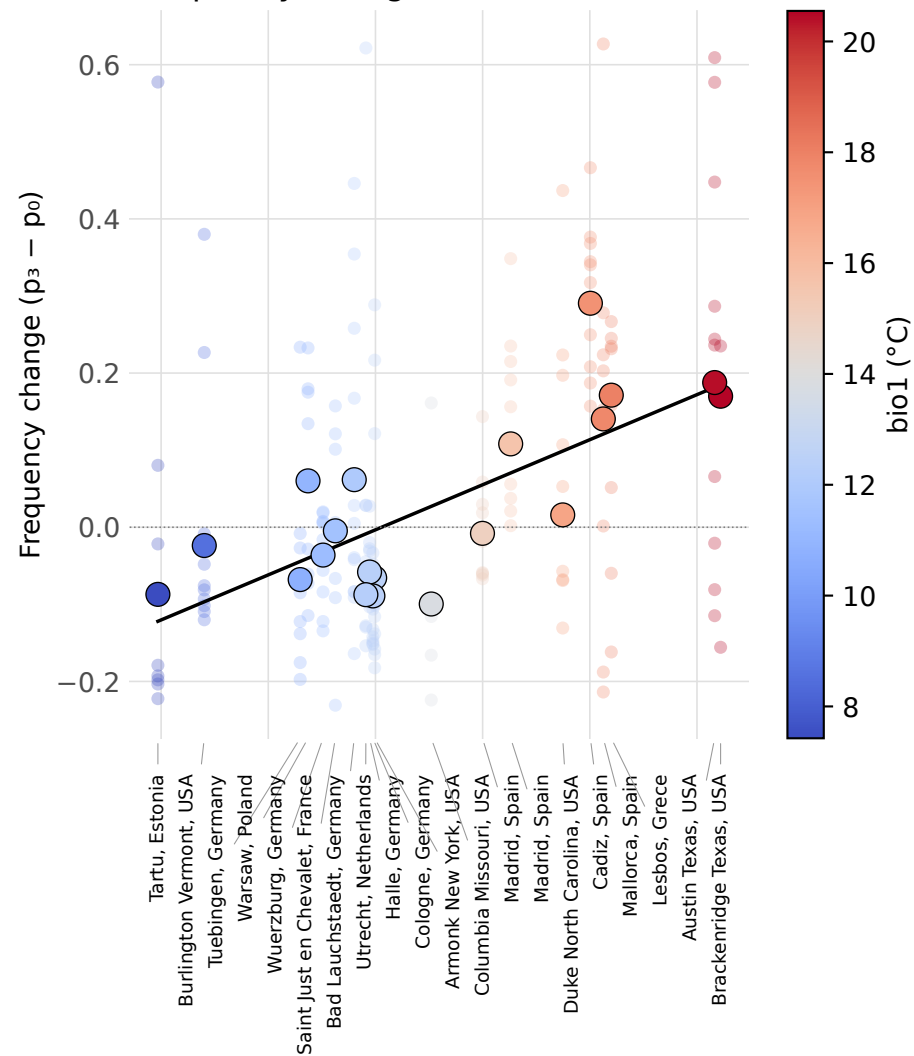
Frequency change vs climate ( r=0.76 )
