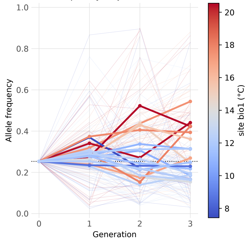
Allele-frequency trajectories (all sites)
