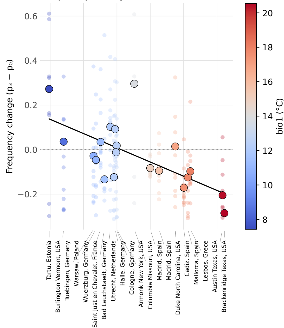
Frequency change vs climate ( r=-0.65 )
