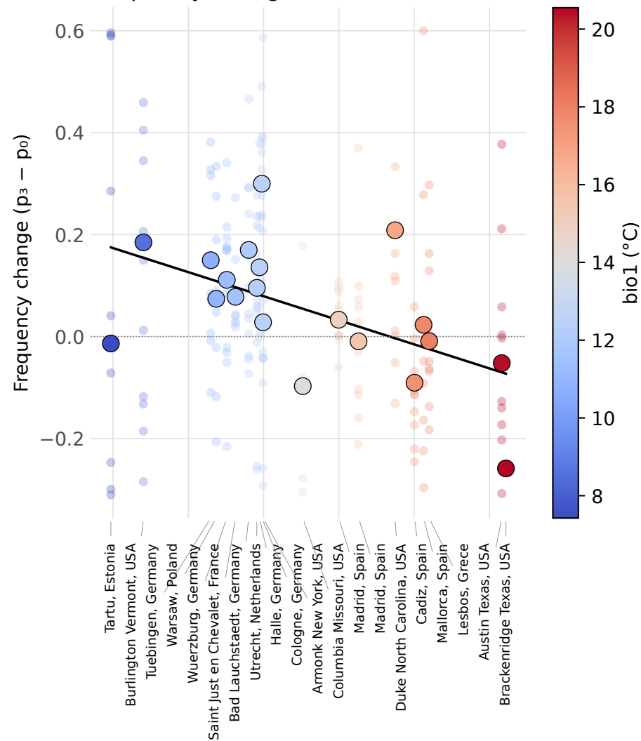
Frequency change vs climate ( r=-0.55 )
