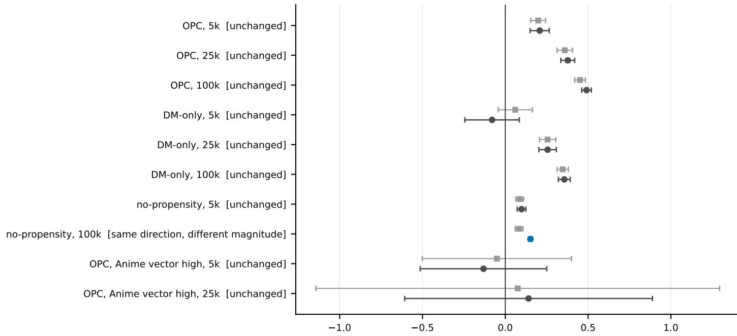
Stage 2: OPC minus each baseline (true CTR points)
