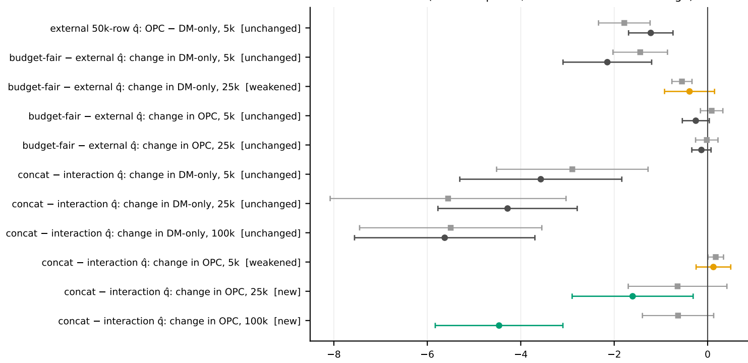
Reward-model tests (true CTR points; combined medium and high)
