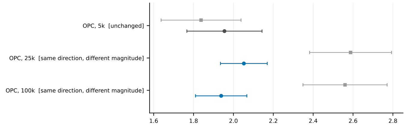
Selected OPC policy's share of weights above 10 (%; biased worlds)
