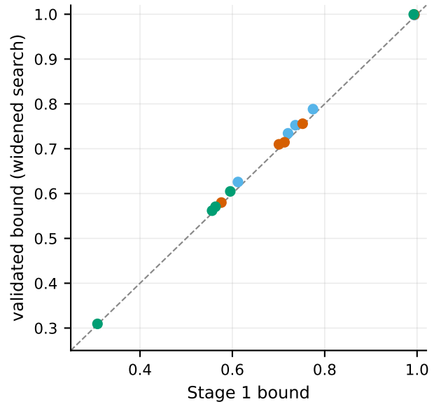
(b) Oracle validation: per dataset \times bias
