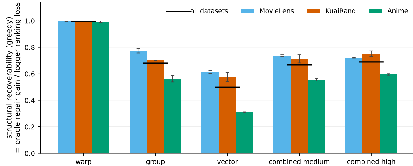
(a) What the linear repair class can recover with the true rewards
