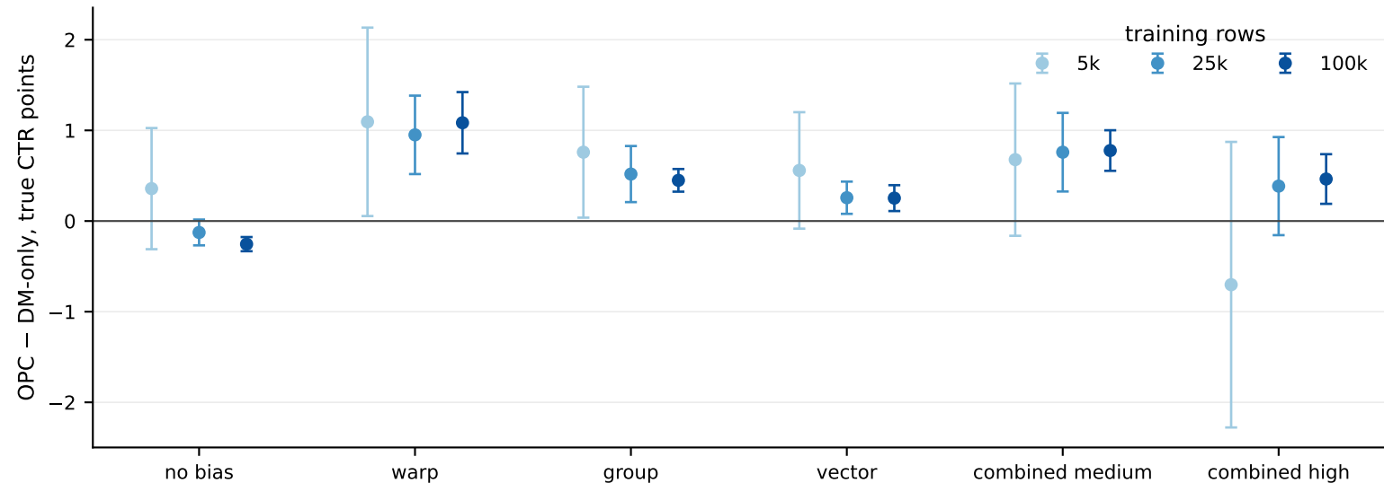
Value of the propensity correction over the reward model alone (paired; mean and 95% CI over 3 datasets \times 2 seeds)
