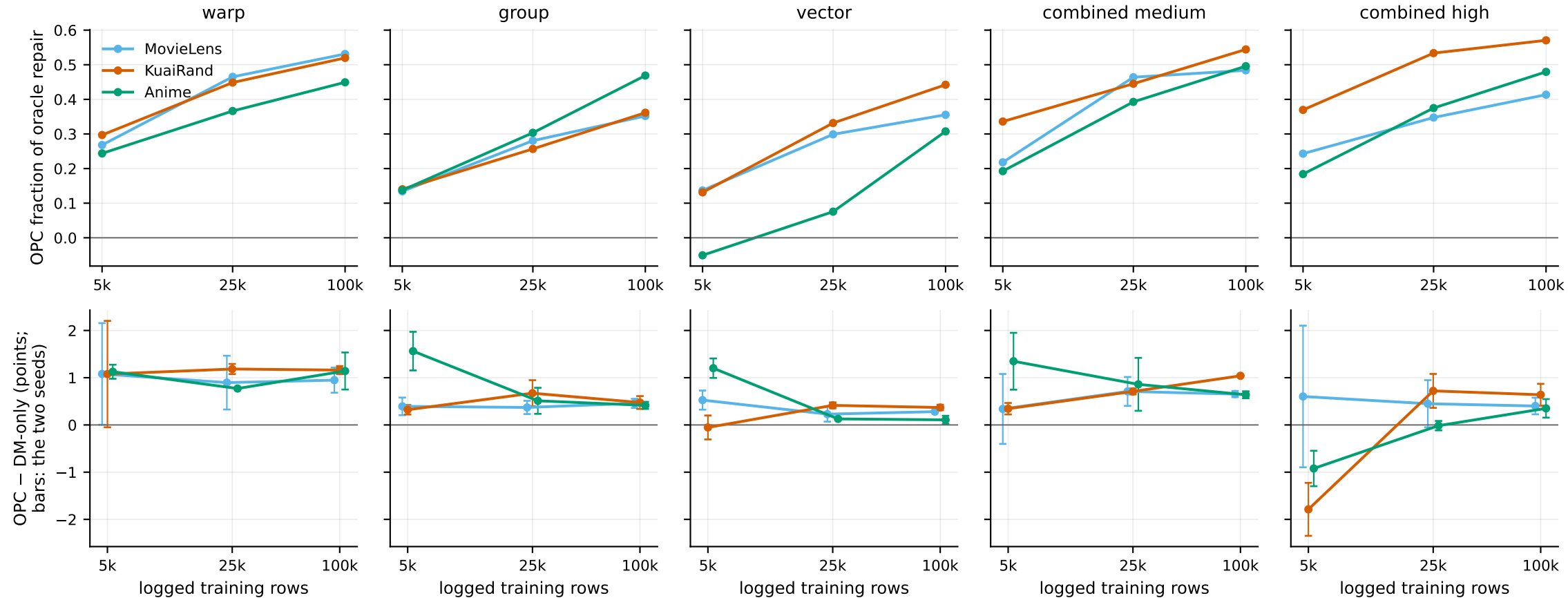
Per dataset (mean of 2 seeds)
