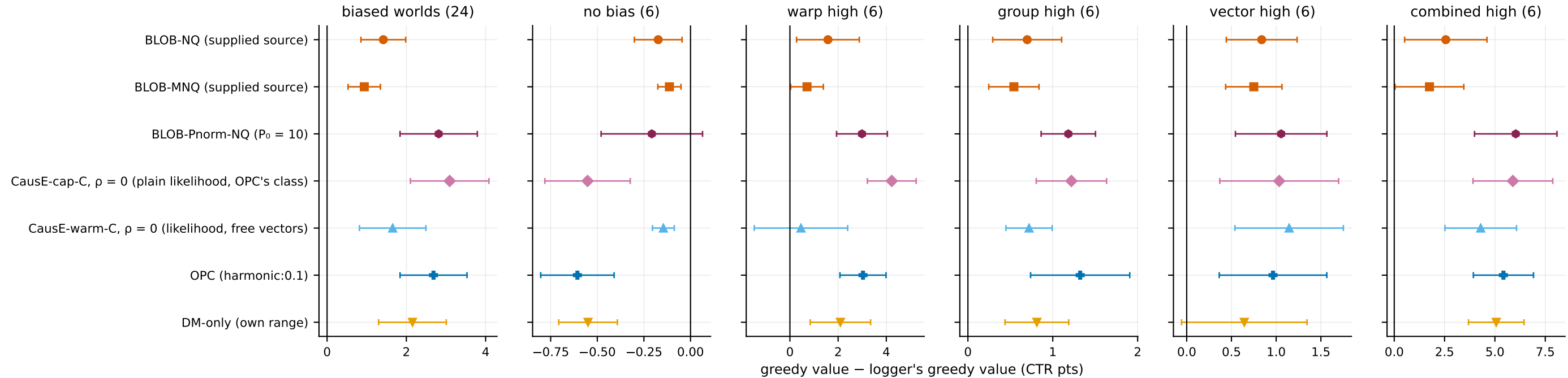
Target value at 25k (mean and 95% CI over worlds); BLOB and the likelihood learners ignore propensities
