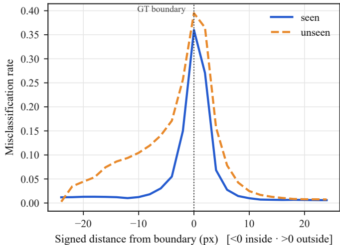
(b) Errors concentrate at the boundary
