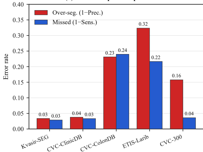
(a) Error composition per dataset
