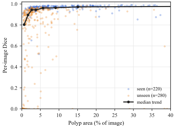
(a) Dice vs. lesion size
