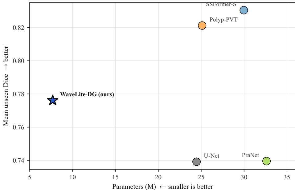
Efficiency vs. generalization (top-left is best)
