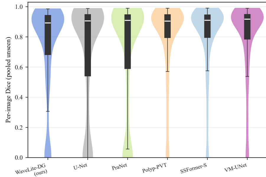
(a) Per-image Dice distribution
