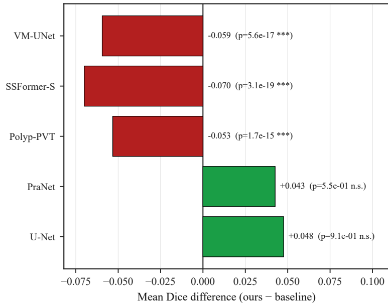
(b) Paired Wilcoxon vs. WaveLite-DG
