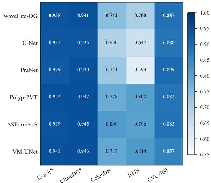
(b) Dice heatmap
