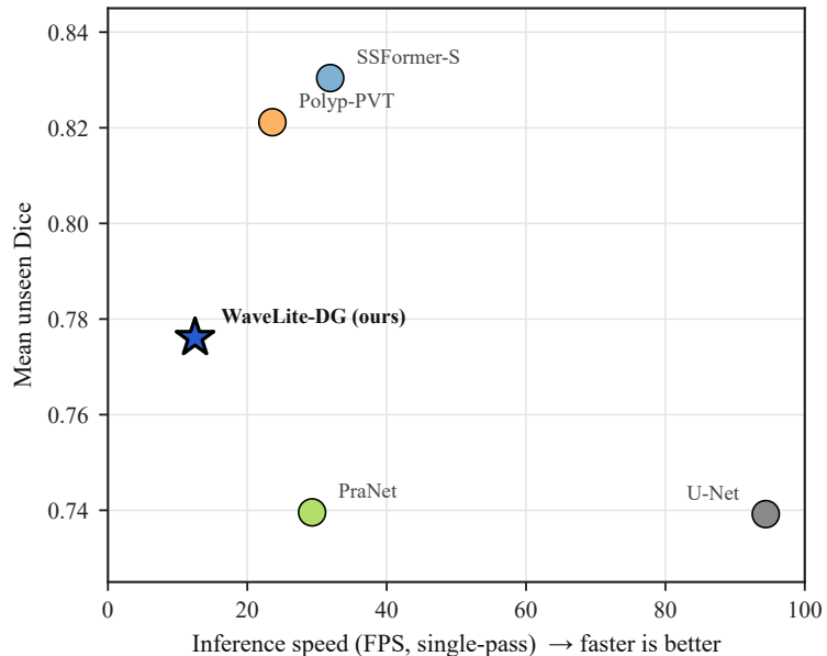
(b) Accuracy vs. speed
