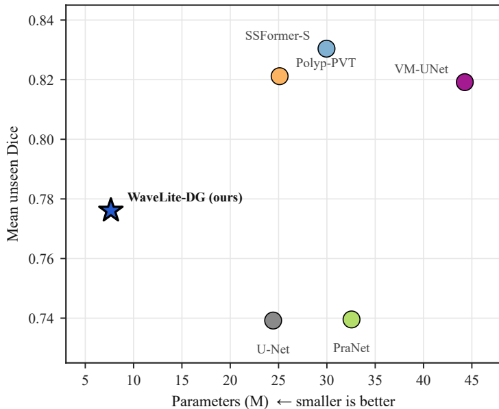
(a) Accuracy vs. model size
