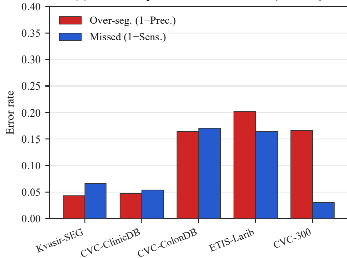
(a) Error composition — SSFormer-S (baseline)
