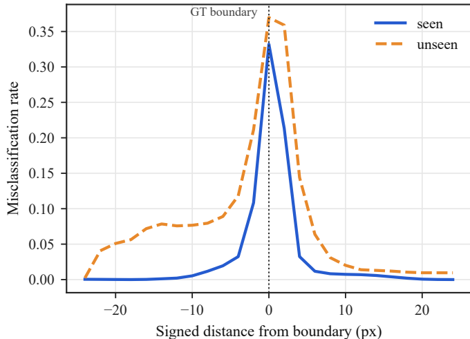
(b) Errors at boundary — SSFormer-S (baseline)
