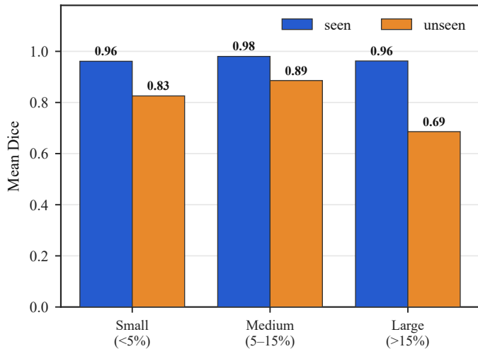
(b) Mean Dice by size — SSFormer-S (baseline)
