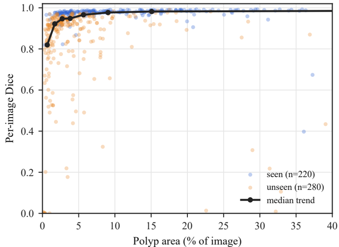
(a) Dice vs. size — SSFormer-S (baseline)
