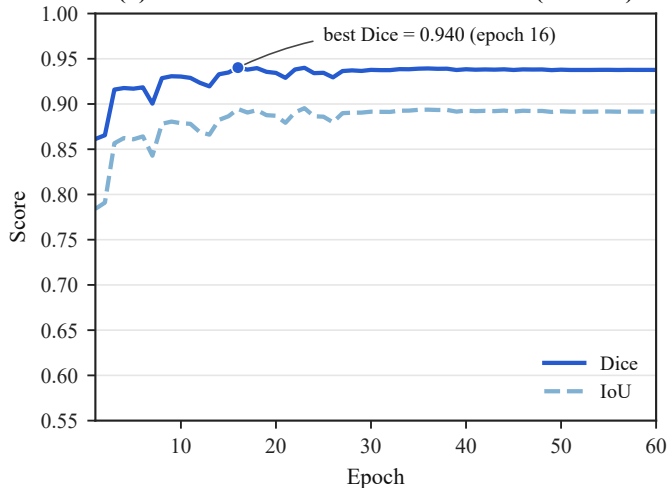
(b) Validation Dice / IoU — SSFormer-S (baseline)
